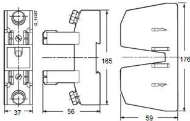
Cylindrical fuse holders KCB20-63A 熔断器底座
